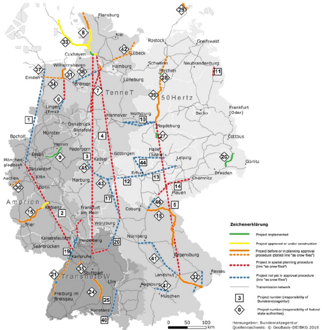
Figure 4: Status of expansion projects in the Federal Requirements Plan Act: 3rd quarter 2017 [26].
