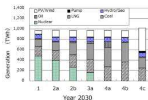
Figure 4.7.3-9: Capacity of each Scenarios Figure 4.7.3-10 : Generation of each Scenarios
