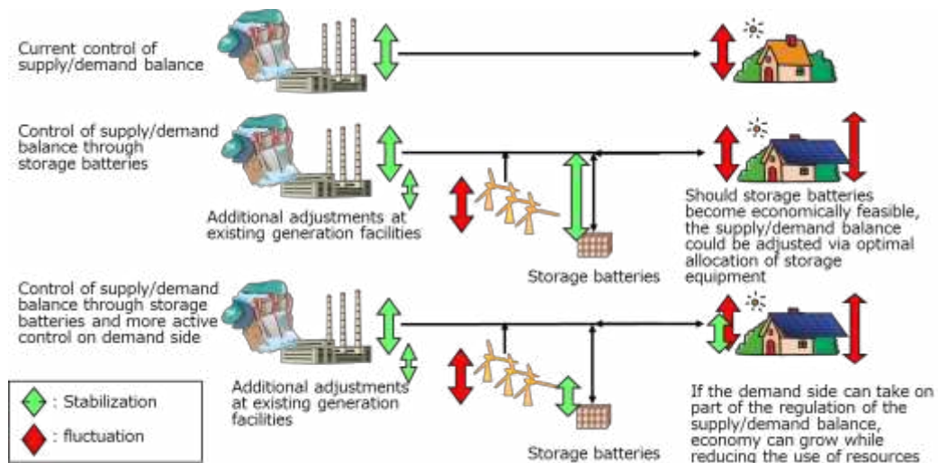
Figure 2.3.1-1: Demand Activation by Distributed EMS
