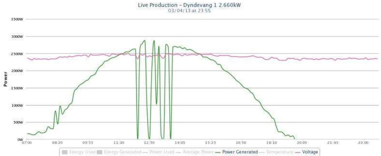
Figure 4.5.3-1: PV generation on 3 rd of April
