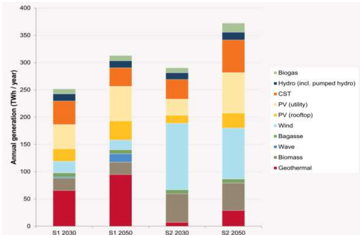
Figure 4.1.4-1: Estimated annual generation of different renewable energy technologies for a 100% renewable sourced NEM in 2030 and 2050 under two different scenarios of future economic growth and technology development progress (AEMO, 2013d).
