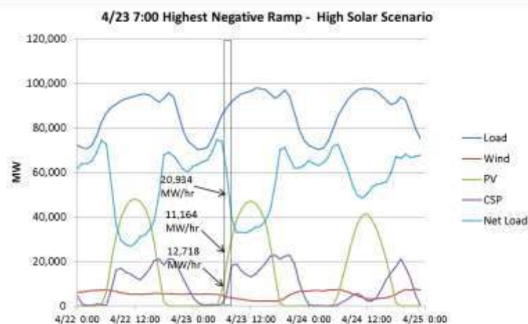
Figure 4.10.3-6: Highest hourly negative ramp (down-ramp) of 20,934 MW in the High Solar Scenario occurs on April 23 at 7:00.
