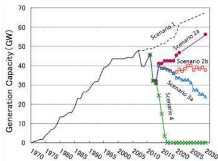
Figure 4.7.3-8: Generation Capacity
