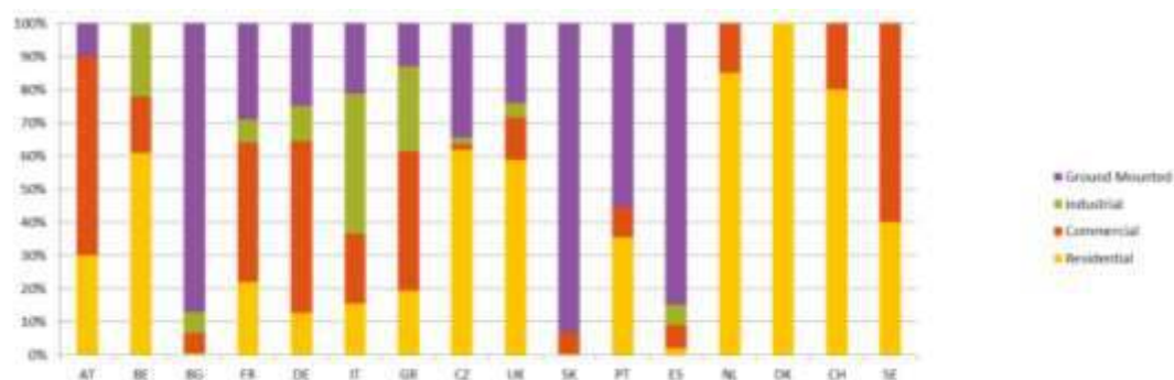
Figure 4.11.2-3: European PV cumulative capacity segmentation in 2012, [2]
