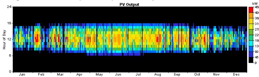
Figure 4.4.3-4b: The power output over the year of the PV system for Scenario 7.
