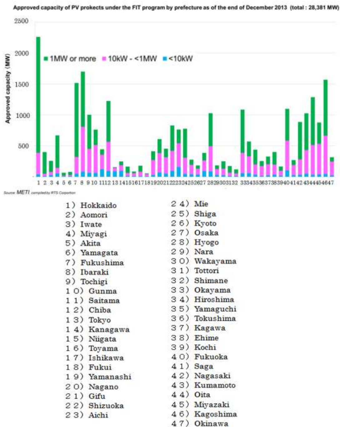
Figure 4.7.2-5: Approved capacities of PV projects under the FIT program by the end of December 2013
