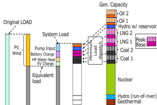
Figure 4.7.3-7 : Minimum load dispatch for Max balancing capability
