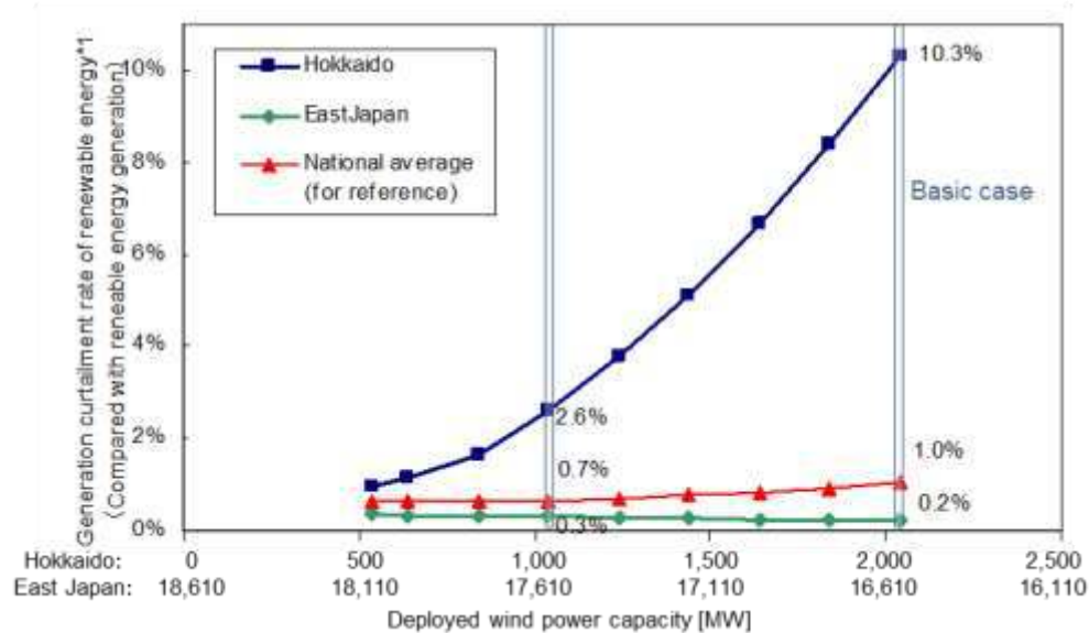
Figure 4.7.3-5: the generation curtailment rate of Hokkaido decreases
