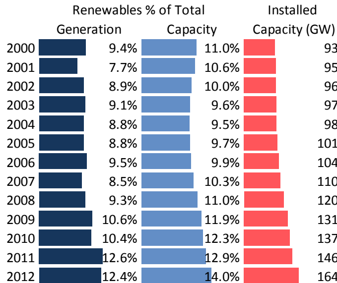
Figure 4.10.2-4: Renewable energy generation and capacity in the U.S. Source: Renewable Energy Data Book, NREL.
