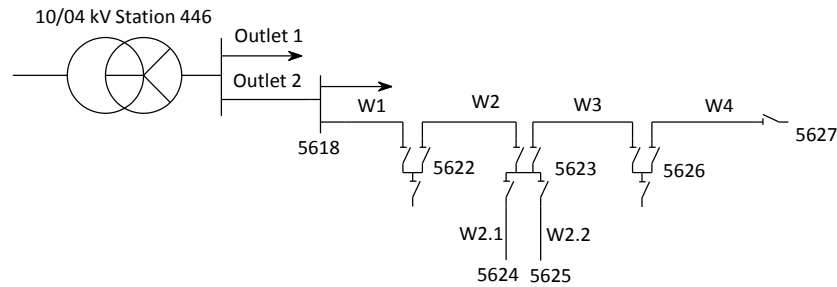
Figure 4.5.3-3: Station 446 diagram
