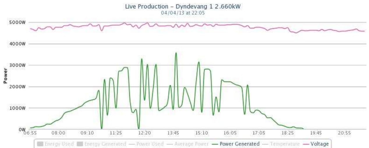
Figure 4.5.3-2: PV generation on 4 th of April
