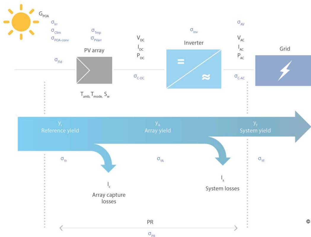
Figure 1: Energy flow diagram in a grid-connected photovoltaic system. In black the calculated parameters and in blue the related uncertainties ( \sigma ).
