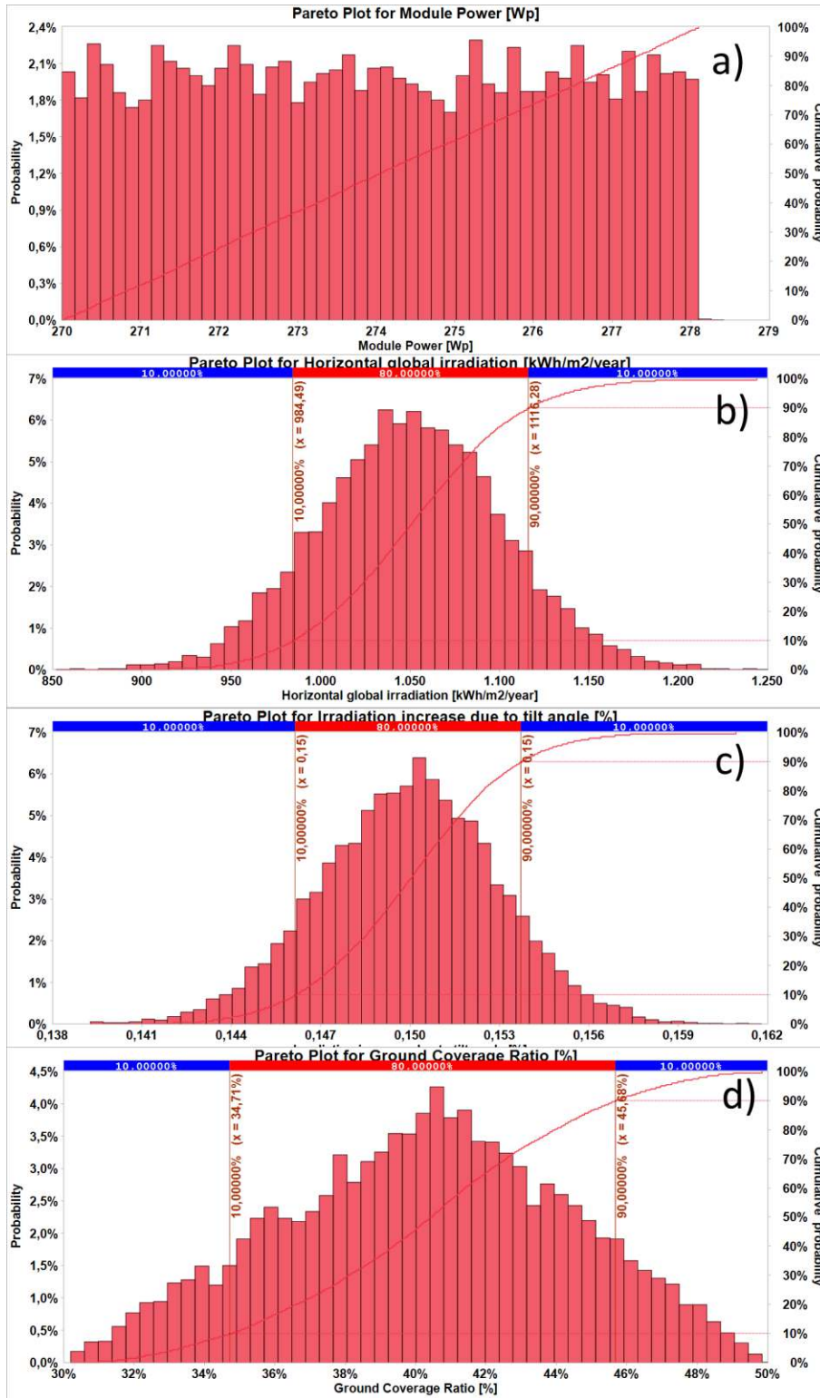
Figure 13: Examples of possible input parameter distributions a) Module power (Uniform) [ W_p ] b) Horizontal global irradiation (Normal) [ kWh/m^2/year ], c) Irradiation increases due to tilt angle (Normal) [%] d) Ground Coverage Ratio (Triangular) [%].
