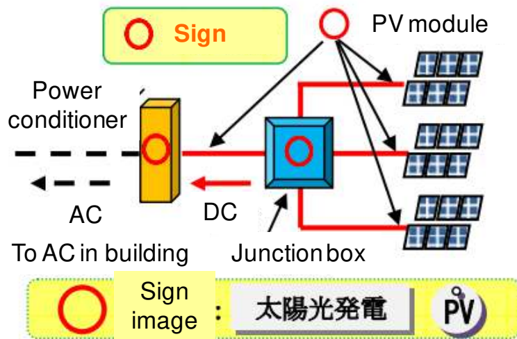
Figure 3.3 Signage rule on a PV system referred to in Tokyo Fire Department directive standards 24 (Translated)
