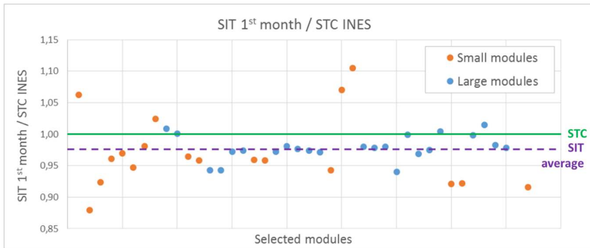
Figure 13: SIT/STC plot for the filtered modules, namely the average of the 150 first power values under an irradiance of 1000 \pm 20 \text{ W/m}^2 corrected at 1000 \text{ W/m}^2 and at 25^\circ\text{C} , divided by the STC power value measured at INES. Small modules ( P < 10 \text{ Wp} ) have been coloured differently as their standard deviation has been observed higher than large modules ( P > 150 \text{ Wp} ). STC = Standard Test Conditions. SIT = Standard Irradiance and Temperature conditions.
