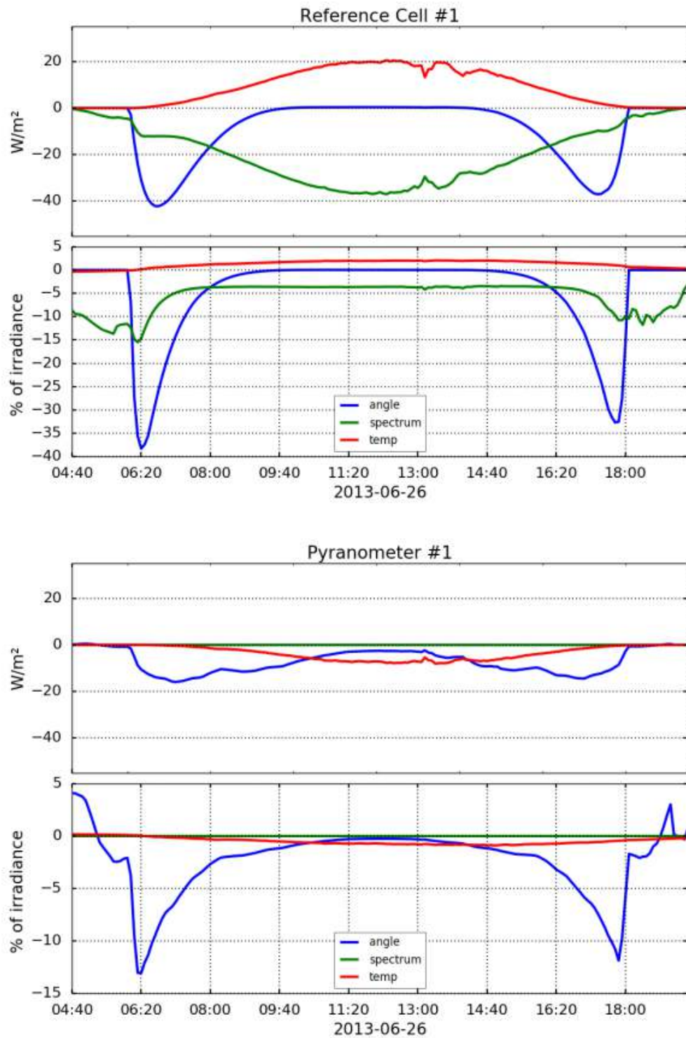
Figure 4: Daily profiles of the measurement error caused by angle-of-incidence, spectrum and temperature for a reference cell and a pyranometer located in Golden Colorado, tilted 40° South.
