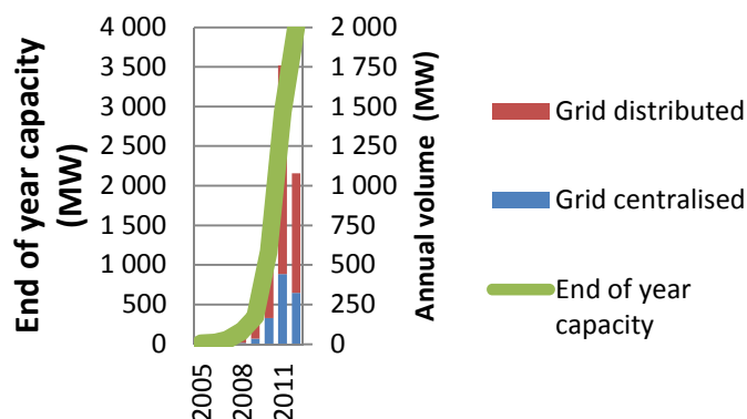
Figure 1 - Annual and cumulated power of grid-connected installations in France
