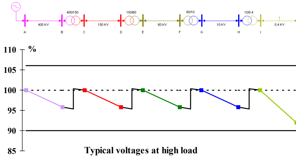
Figure 2 Voltage limits and typical voltages at high load in a classic power system
