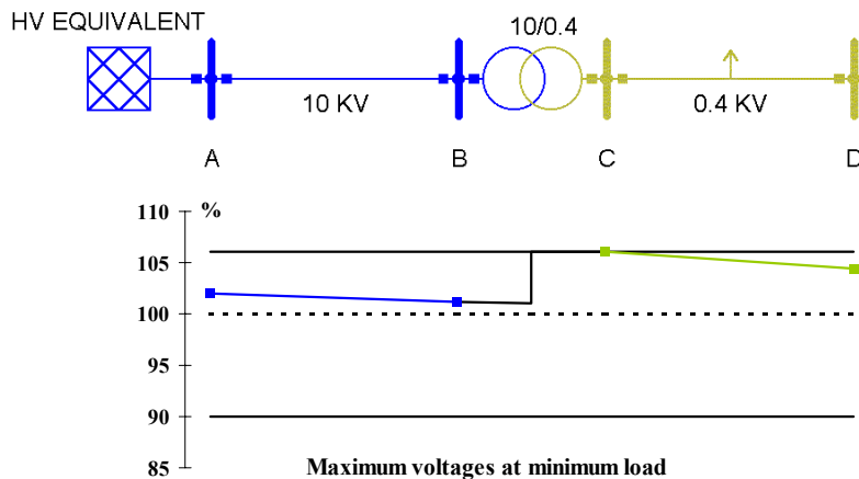
Figure 7 Maximum voltages at minimum load in the simplified power system
