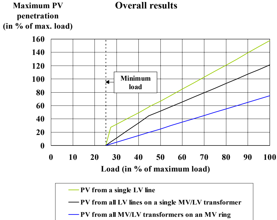
Figure 14 Overall limits of PV penetration into existing power systems
