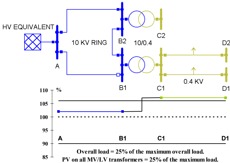
Figure 13 An amount of PV penetration equal to the load from all five MV/LV transformers of a half MV ring causes an over-voltage of 106.6% at minimum load
