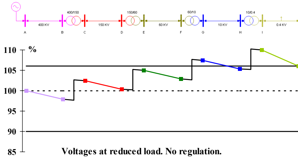
Figure 3 Voltages at reduced load if no voltage regulation is applied
