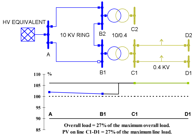
Figure 10 An amount of PV penetration equal to the load is acceptable at 27% of the maximum load
