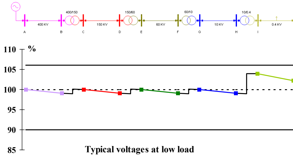
Figure 4 Voltages at low load if voltage regulation is applied
