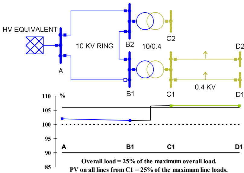
Figure 12 An amount of PV penetration equal to the load from all the 5 LV lines from an MV/LV transformer causes an over-voltage of 106.6% at minimum load
