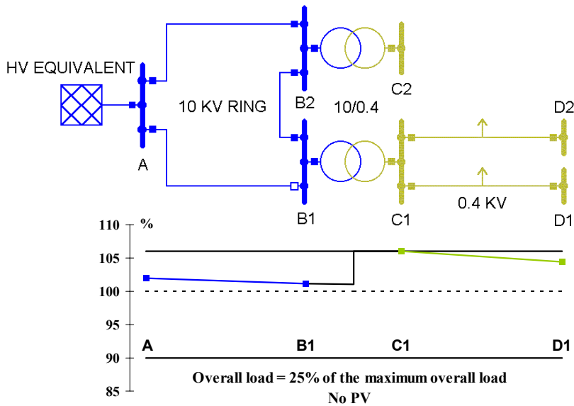
Figure 9 No PV is acceptable at minimum load (25% of maximum load)
