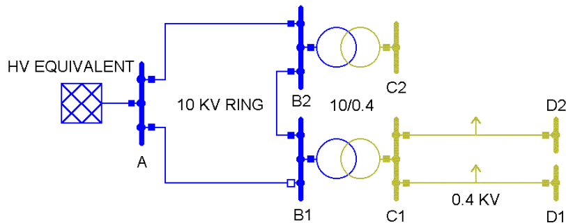
Figure 8 Typical configuration of the MV/LV power system
