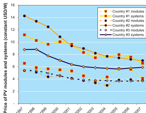
Figure 10 – Evolution of price of PV modules and systems in selected reporting countries accounting for inflation effects – Years 1997–2007
