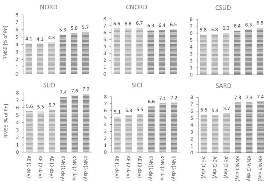
Figure 20: RMSE of the PV power forecasts of each market zone obtained by the AE and KNN models at different horizons.
