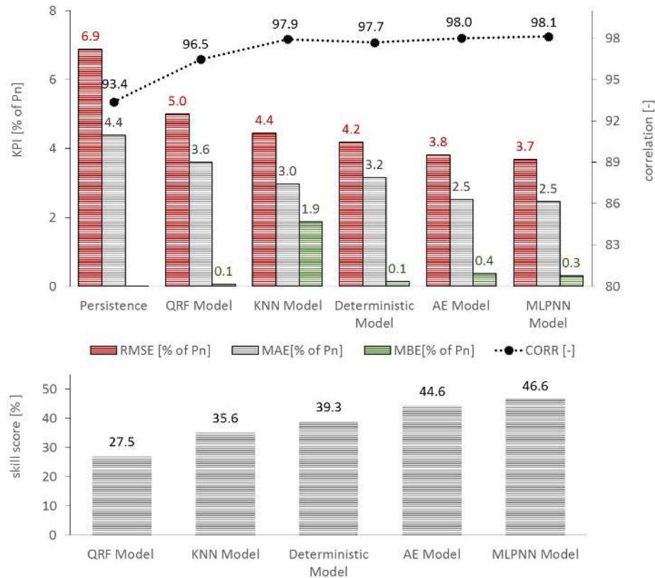
Figure 26: Main Key Performance Indexes (KPIs) of the forecasts.
