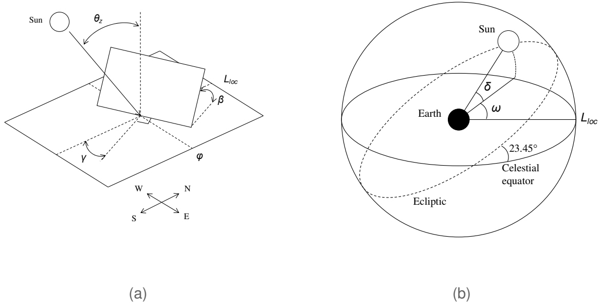
Figure 1: In (a), the relevant angles (plane tilt \beta , azimuth angle \gamma , latitude \phi , longitude L_{loc} and zenith angle \theta_z ) that define the location and orientation of the tilted plane. In (b), the relevant angles (hour angle \omega and solar declination \delta ) defining earth's position relative to the sun that constitute the deterministic variability. Combined, these can be used to calculate the angle of incidence \theta and subsequently the plane irradiance. Copied with permission of the copyright owners [10].
