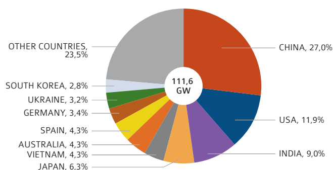
FIGURE 2.5: GLOBAL PV MARKET IN 2019
