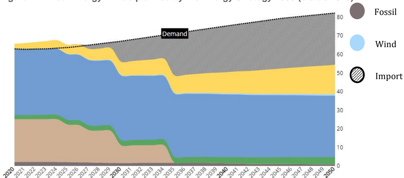
Figure 8 Annual Energy Mix evolving at the current pace if the rates are stable from 2020 on (status 2020)
