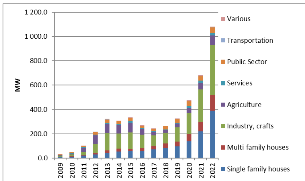
Figure 1: Photovoltaic installed capacity per sector
