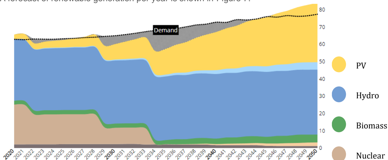
Figure 7 Annual Energy Mix as planned by the Energy Strategy 2050 (status 2020)
