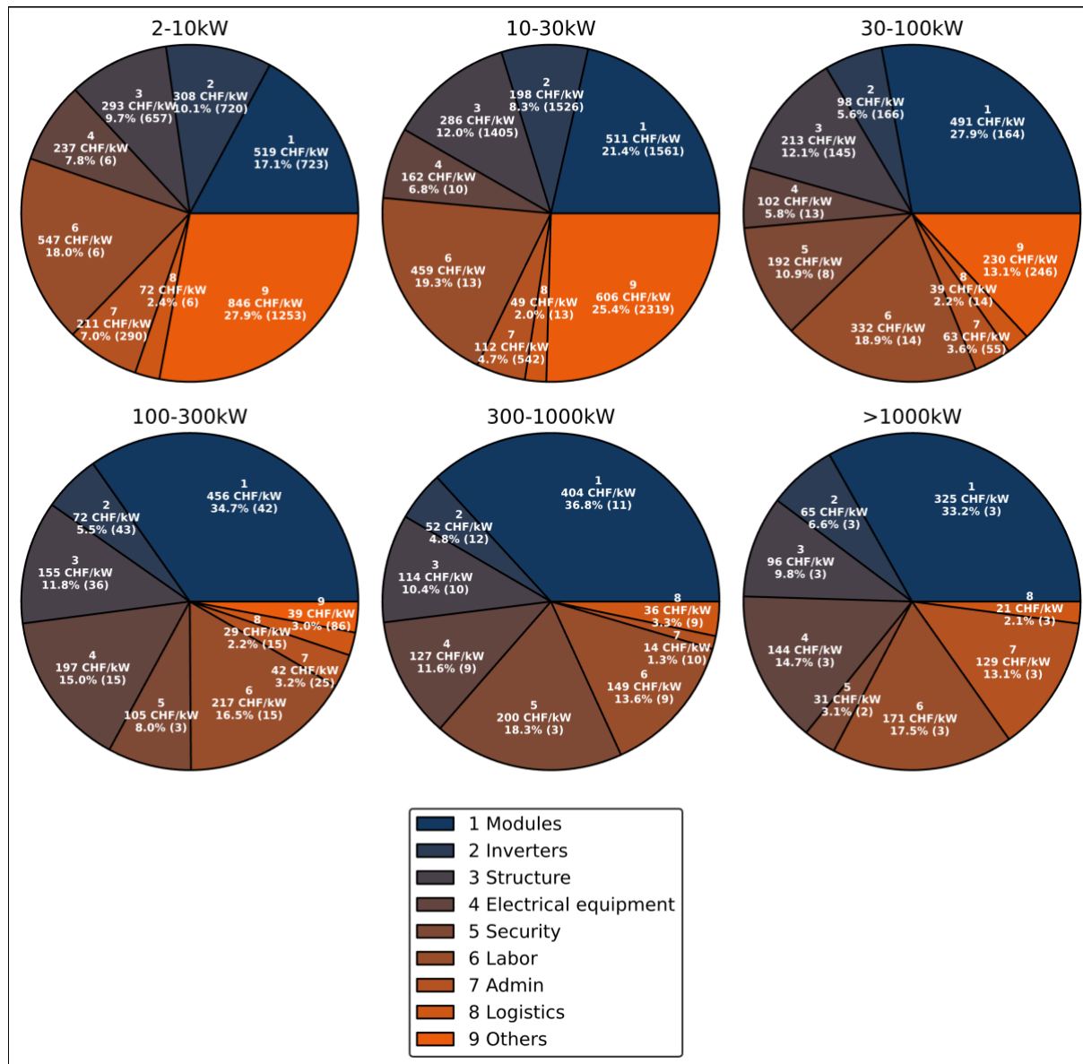
Figure 5 : Cost breakdown of BAPV in 2022 (source: Observation des prix du marché photovoltaïque 2022)
