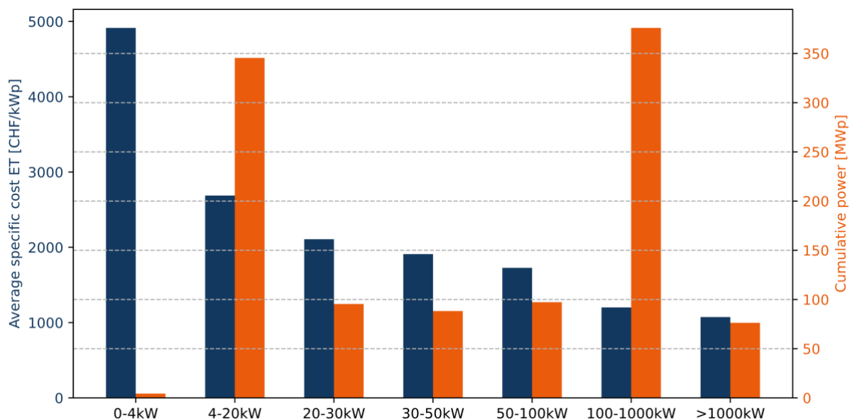
Figure 11 : Average specific cost and cumulative power for each power category
