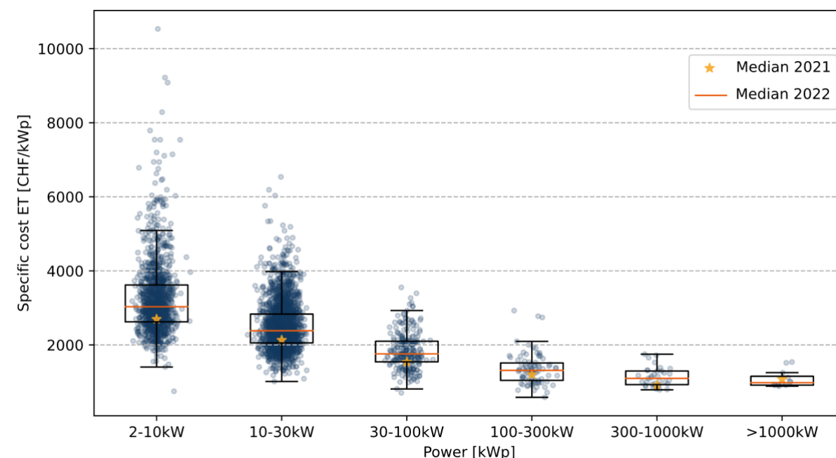
Figure 4 : Grid-connected PV system specific costs (source: Observation des prix du marché photovoltaïque 2022)
