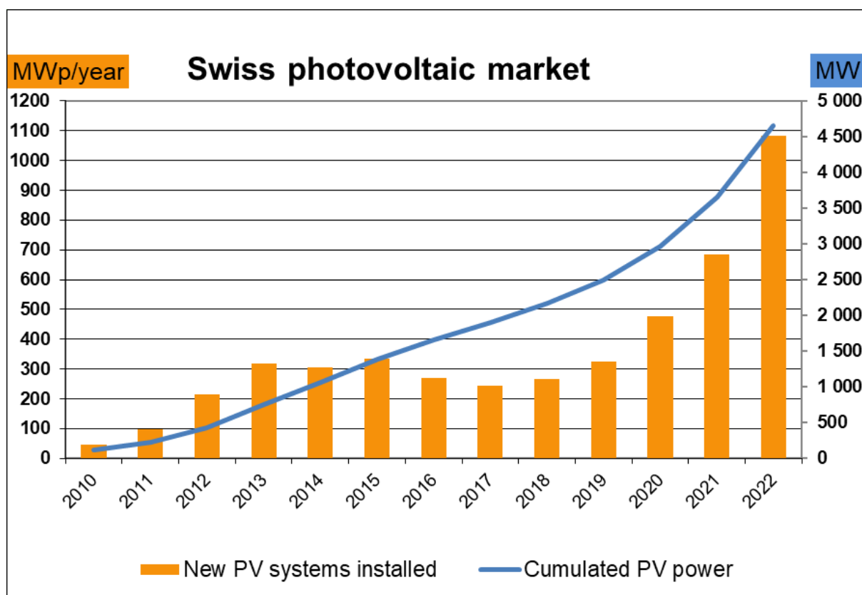
Figure 3 Installed PV capacity per year
