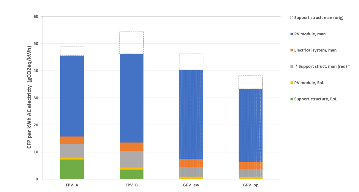
Figure 9: Carbon footprint per kWh AC electricity: support structure with recycled materials. 17
