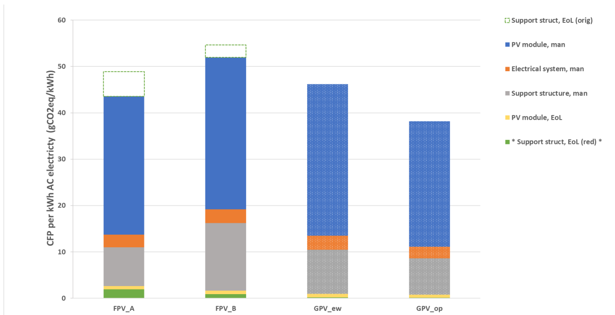
Figure 10: Carbon footprint per kWh AC electricity: support structure with improved end-of-life treatment. 18
