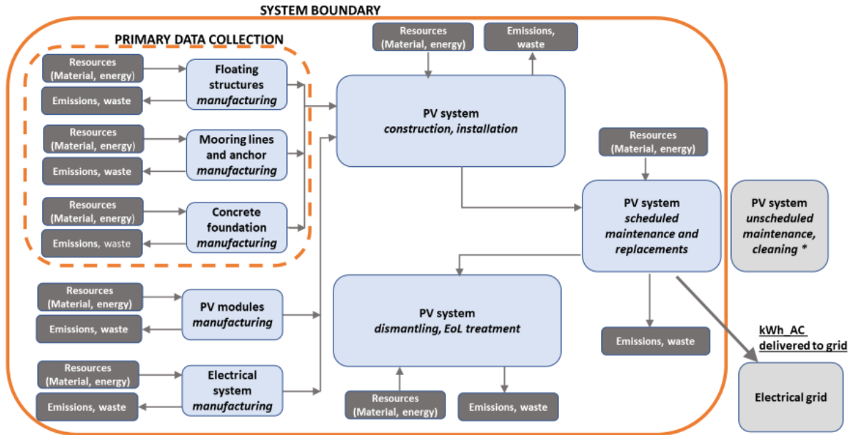
Figure 1: Flow diagram with system boundary.
