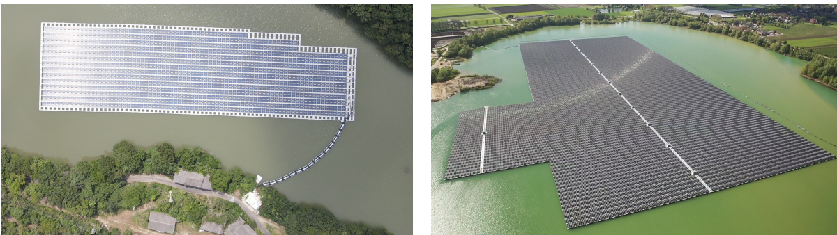
Figure 2: Aerial pictures of both floating PV systems (left: FPV_A, right: FPV_B).
