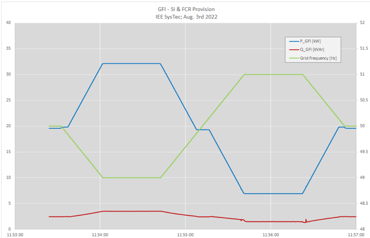
Figure 13: Provision of Synthetic Inertia response (Spinning Reserve) and Frequency Containment Reserve (P) as well as Reactive Power Q of the GFI in the PNI lab in case of rampwise network frequency variations
