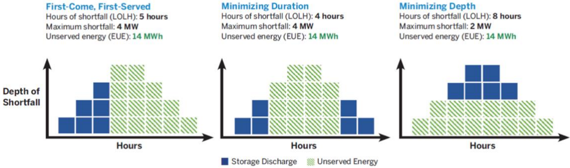
Figure 4.4. Battery storage scheduling can influence resource adequacy metrics. (Source: ESIG, 2024, https://www.esig.energy/new-resource-adequacy-criteria ).
