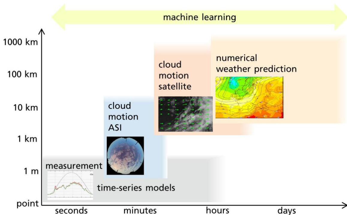
Figure 2.6 Different forecasting methods suitable for various spatial and temporal scales.
