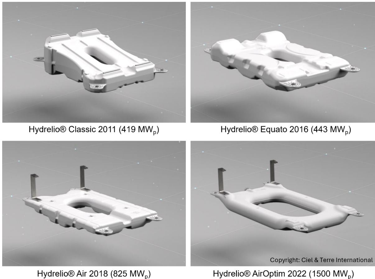
Figure 6. Development of Ciel & Terre Hydrelion® technology. The numbers refer to accumulated installed capacity for Ciel & Terre up until the given year. Copyright: Ciel & Terre International.
